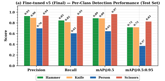
FIGURE 19. Full per-class metrics (precision, recall, mAP@0.5, mAP@0.5:0.95) for the deployed v5 model.
