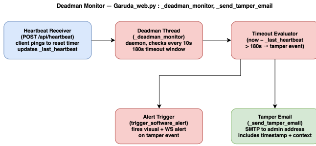
FIGURE 13. Deadman monitor. 10 s wake, 180 s heartbeat deadline, and parallel tamper-alert and email branches on violation.
