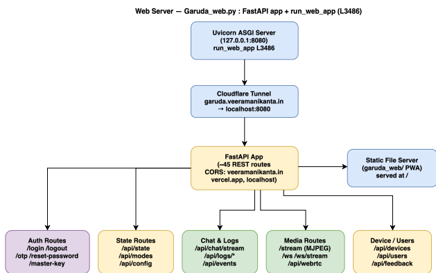
FIGURE 11. Web server. FastAPI under Uvicorn behind a Cloudflare tunnel, with ~45 REST routes and three parallel media channels (MJPEG, WebSocket, WebRTC).
