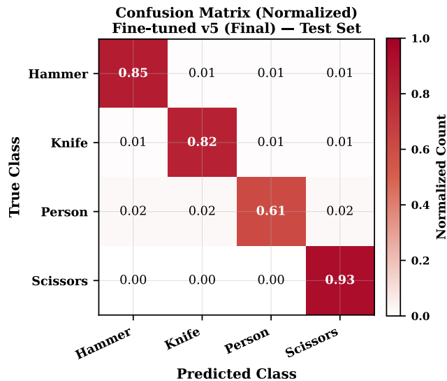
FIGURE 20. Normalised confusion matrix on the v5 held-out test set. Diagonal dominance confirms strong per-class discrimination, with inter-class confusion \leq 0.03 .
